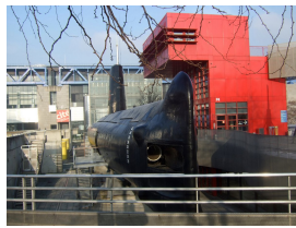
Argonaute
